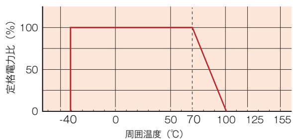
○ PXV1220S, PBV1632S
