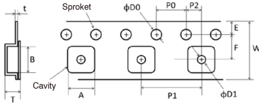
Fig.3 Embossed tape 8mm pitch
