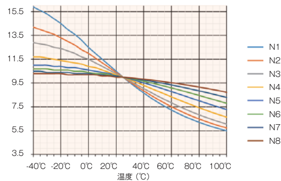
PXV1220S-10dB-N*
