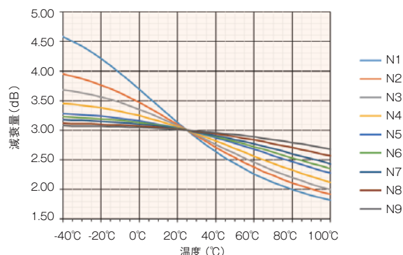
PXV1220S-3dB-N*
