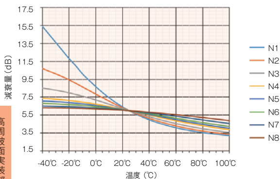
PXV1220S-6dB-N*
